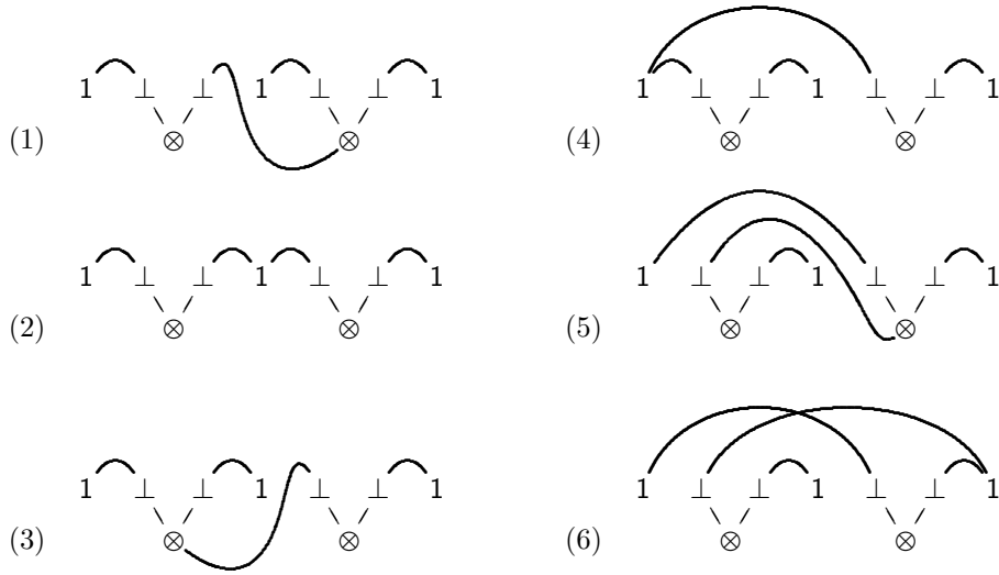
Figure 1: Different representations of the same proof
