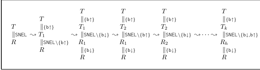
Figure 4: Permuting b\uparrow up and b\downarrow down
