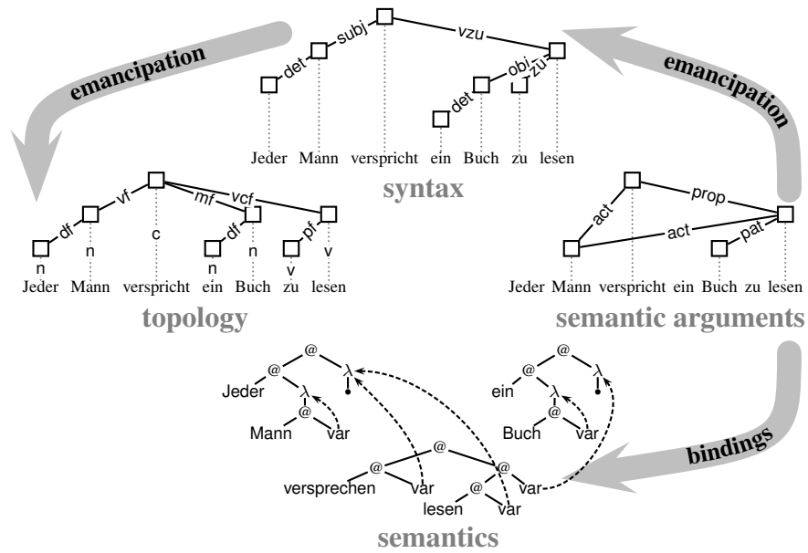
Figure 1: An architectural overview of extended TDG
