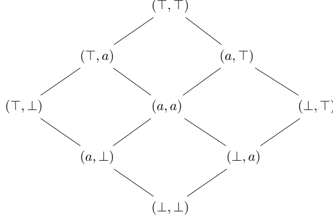
Figure 4: The partial order for H_3
